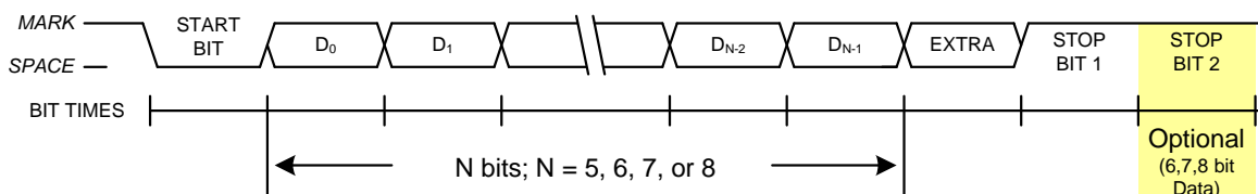
Figure 22.4. UART0 Timing With Extra Bit
