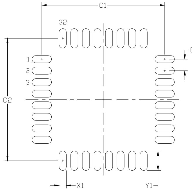
Figure 3.8. QFP-32 Landing Diagram
