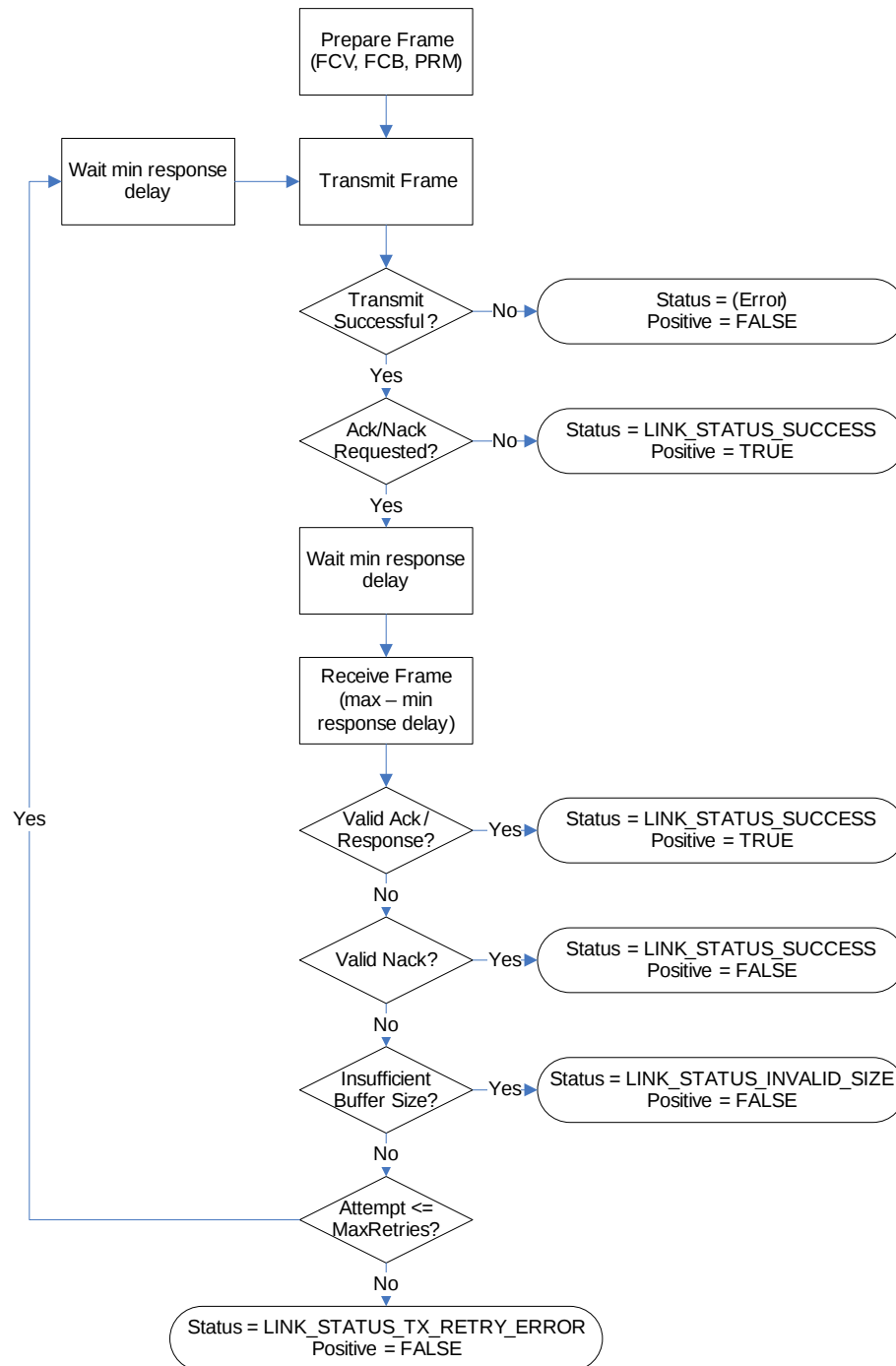
Figure 2. MbusLinkServicesRequest Flowchart
