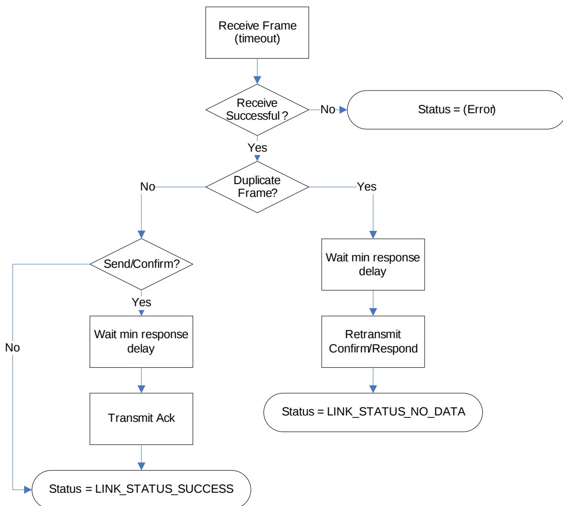
Figure 3. MbusLinkServicesIndication Flowchart
