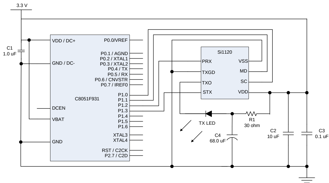
Figure 2. Si1120 Circuit
