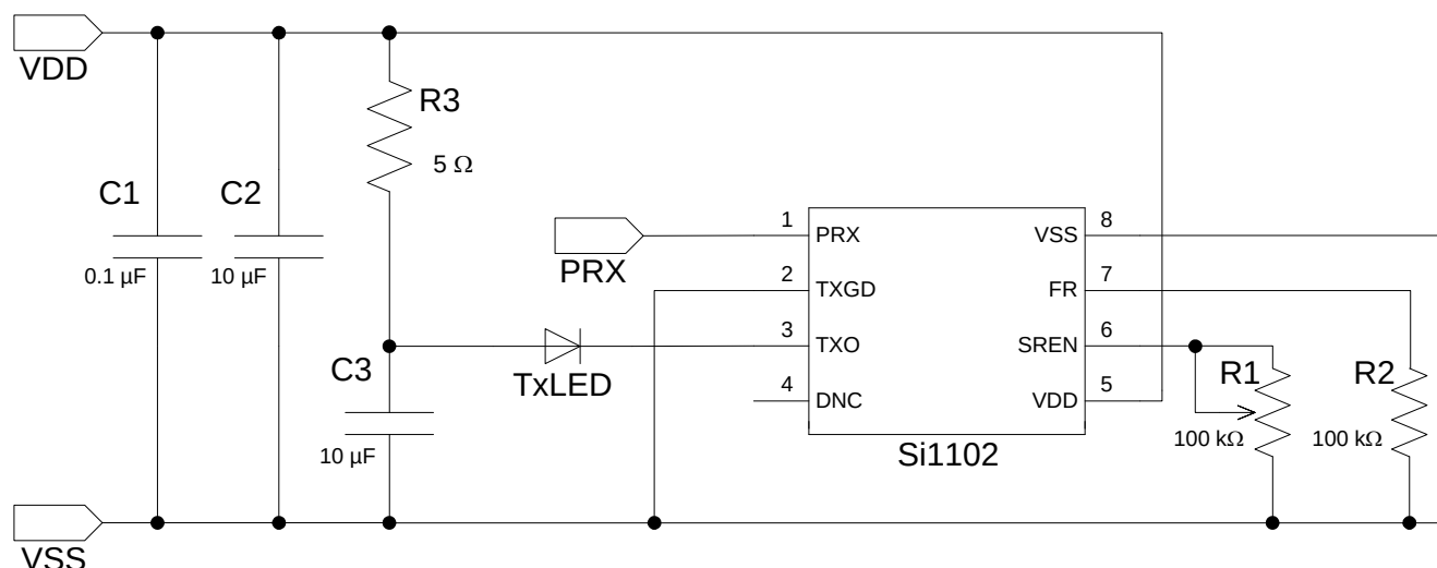
Figure 3. Si1102 Circuit
