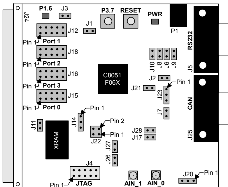
Figure 3. C8051F060 Target Board
