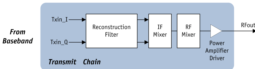
Figure 7-3. Radio Transmit Chain Block Diagram
