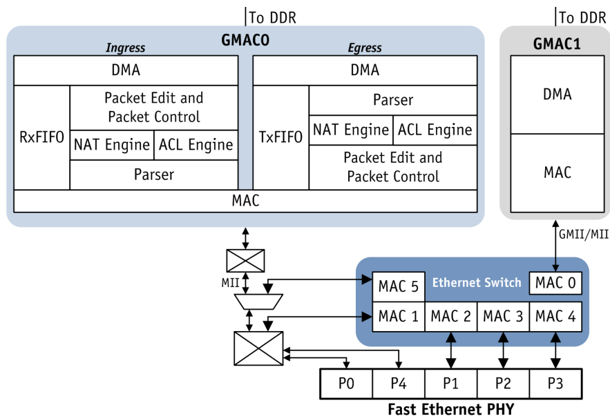
Figure 4-1. Ethernet Subsystem
