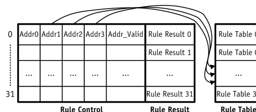
Figure 4-5. ACL Rule Architecture
