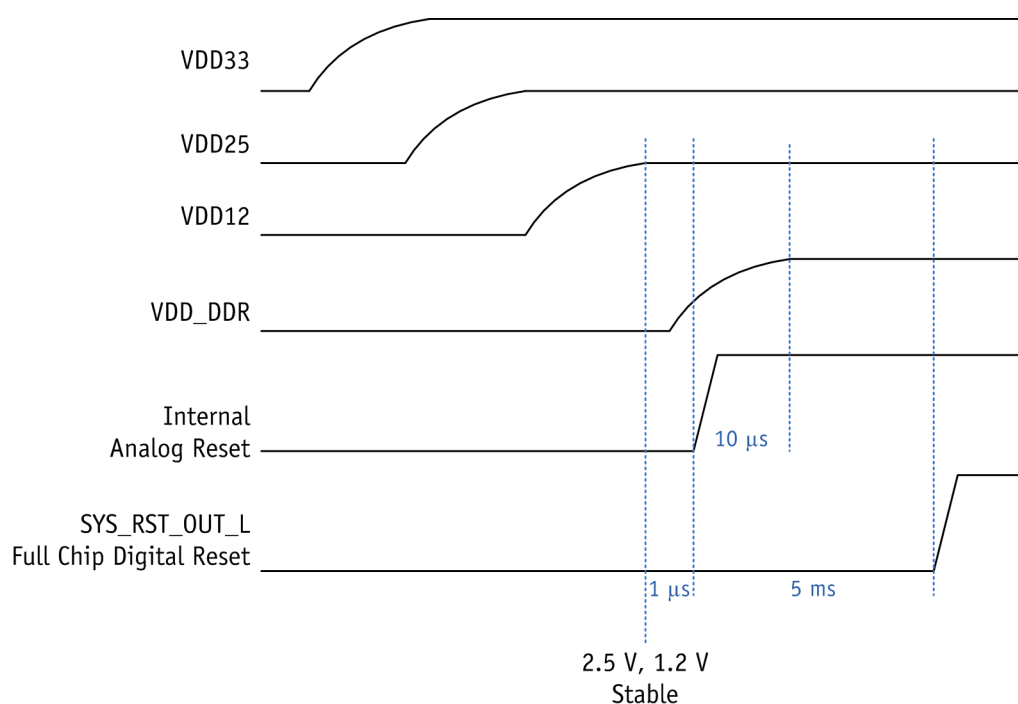
Figure 10-4. Example Reset Timing
