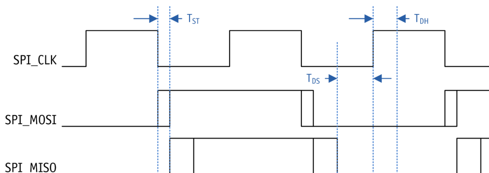
Figure 10-3. SPI Timing
