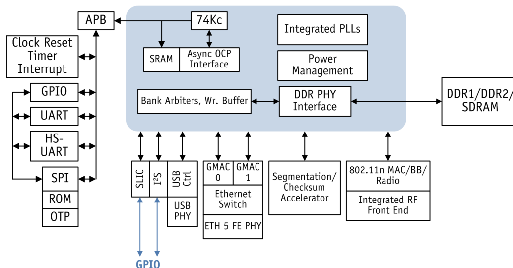
Figure 2-1. AR9341 Functional Block Diagram
