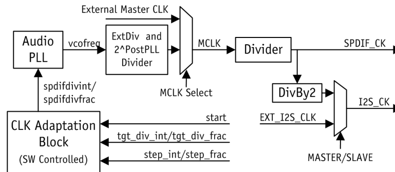
Figure 3-2. Audio PLL Block Diagram
