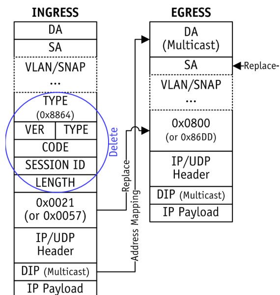
Figure 4-6. PPPoE Header Removal
