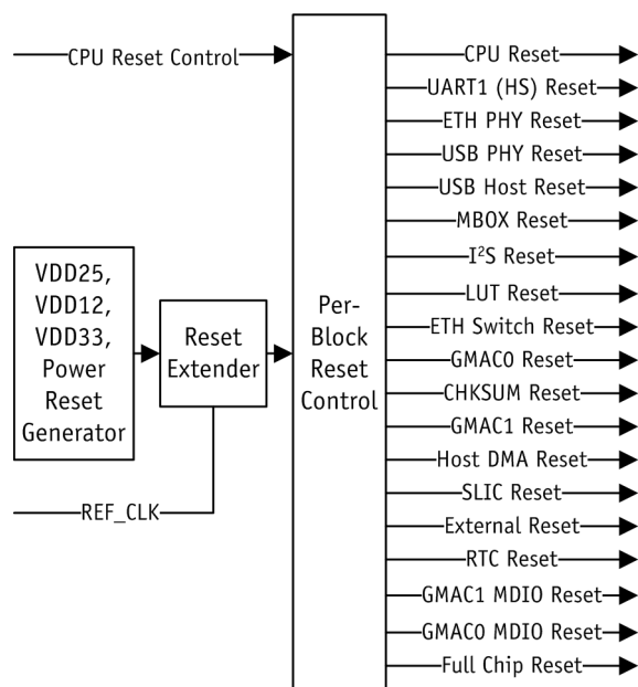
Figure 2-2. AR9341 Reset
