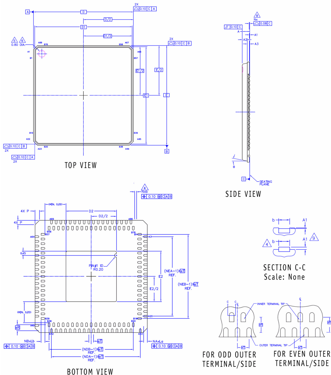
Figure 11-1. AR9341 Package Drawing
