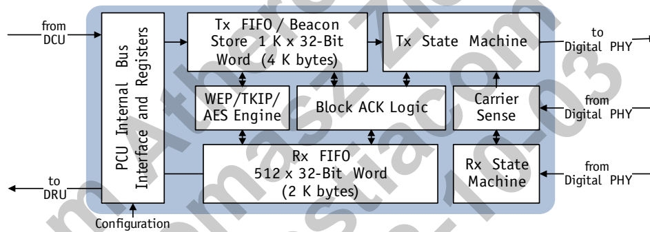
Figure 4-2 PCU Functional Block Diagram
