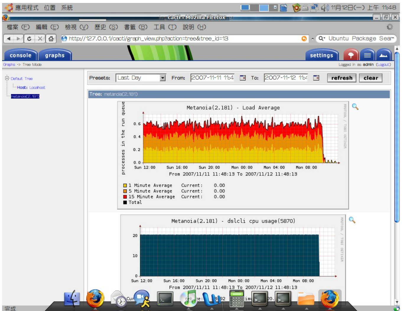
GUI interface
