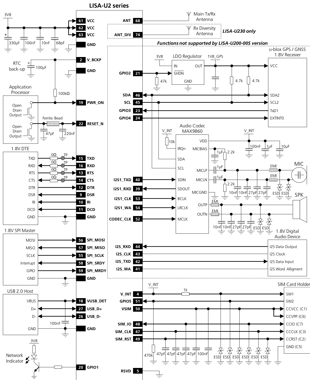
Figure 55: Example of schematic diagram to integrate LISA-U2 series modules in an application board, using all the interfaces
