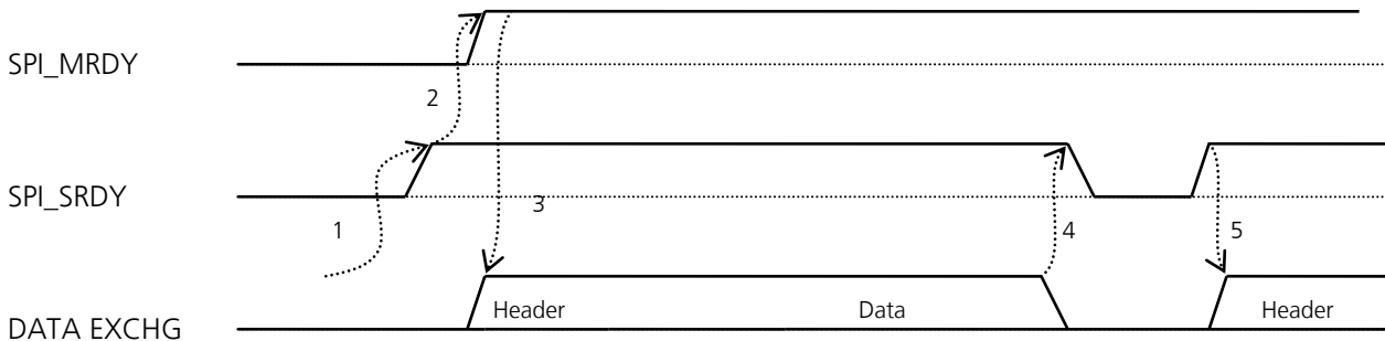
Figure 36: Data transfer initiated by LISA-U module (slave), with a sleeping application processor (master)
