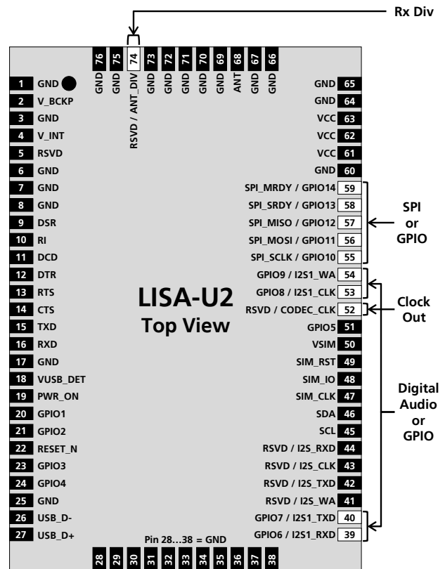
Figure 79: LISA-U2 series pin assignment (highlighted name/function changes)
