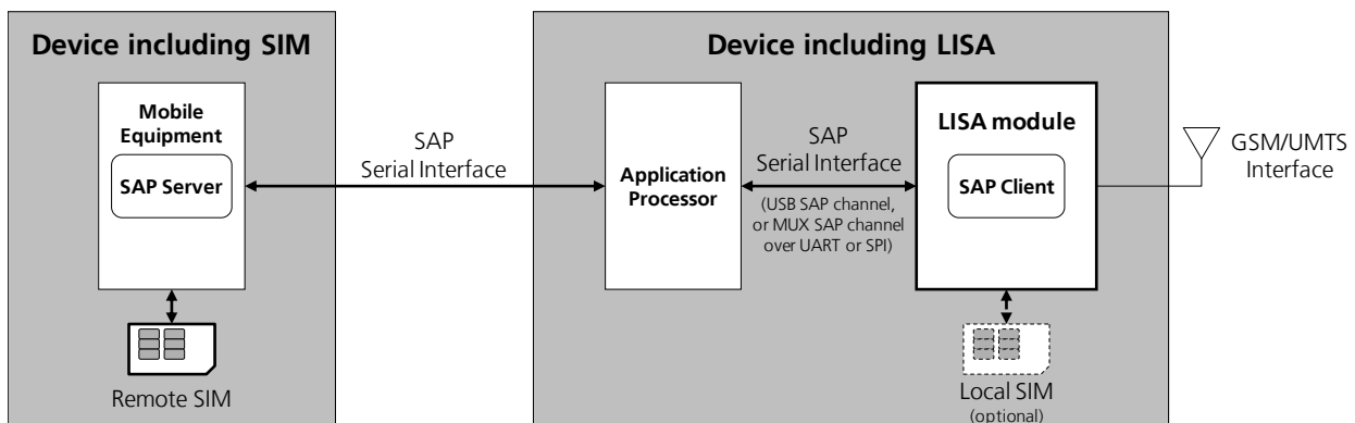
Figure 73: Remote SIM access via completely wired connection
