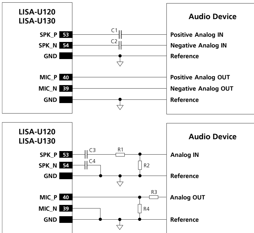
Figure 46: Application circuits to connect the module to audio devices with proper differential or single-ended input/output
