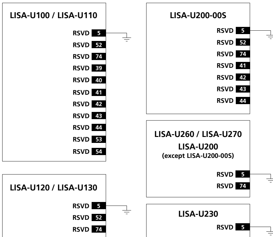
Figure 53: Application circuit for the reserved pins (RSVD)
