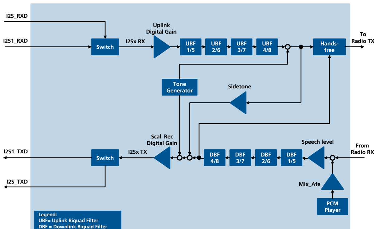
Figure 50: Audio processing system of all LISA-U2 series modules except LISA-U200-005
