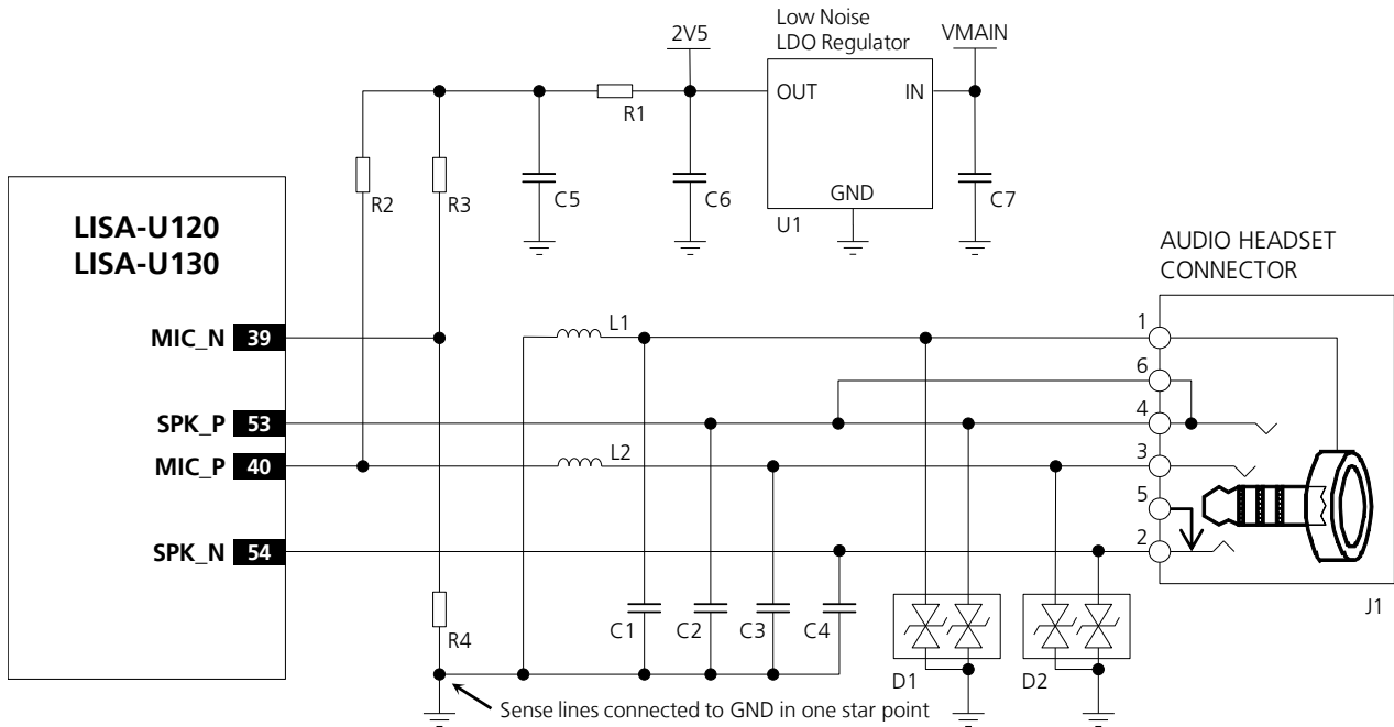
Figure 43: Headset mode application circuit
