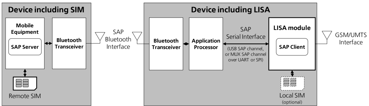
Figure 74: Remote SIM access via Bluetooth and wired connection
