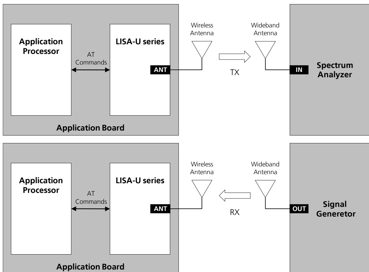
Figure 77: Setup with spectrum analyzer and signal generator for radiated measurement
