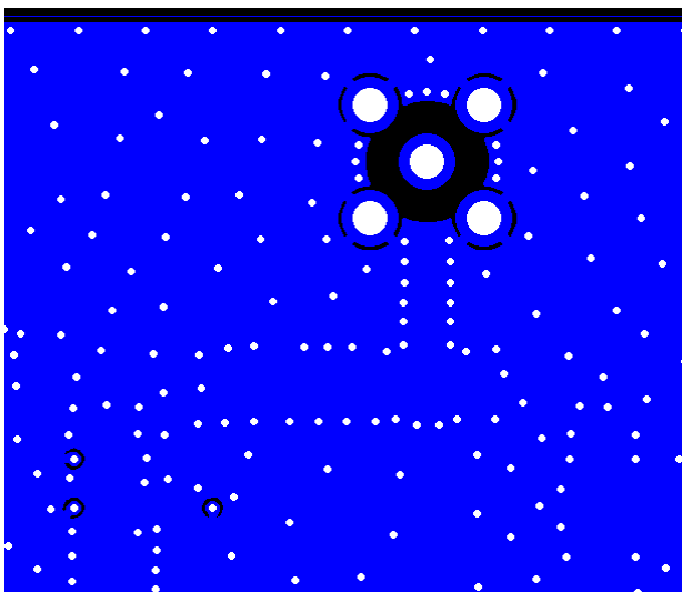
Figure 59: Layer 2 (inner layer) of u-blox approved interface board for LISA-U modules
