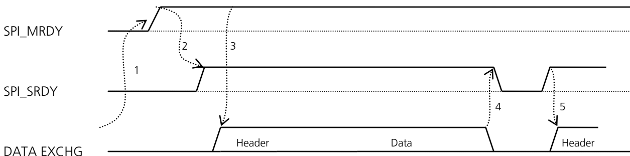
Figure 37: Data transfer initiated by application processor (master) with a sleeping LISA-U module (slave)
