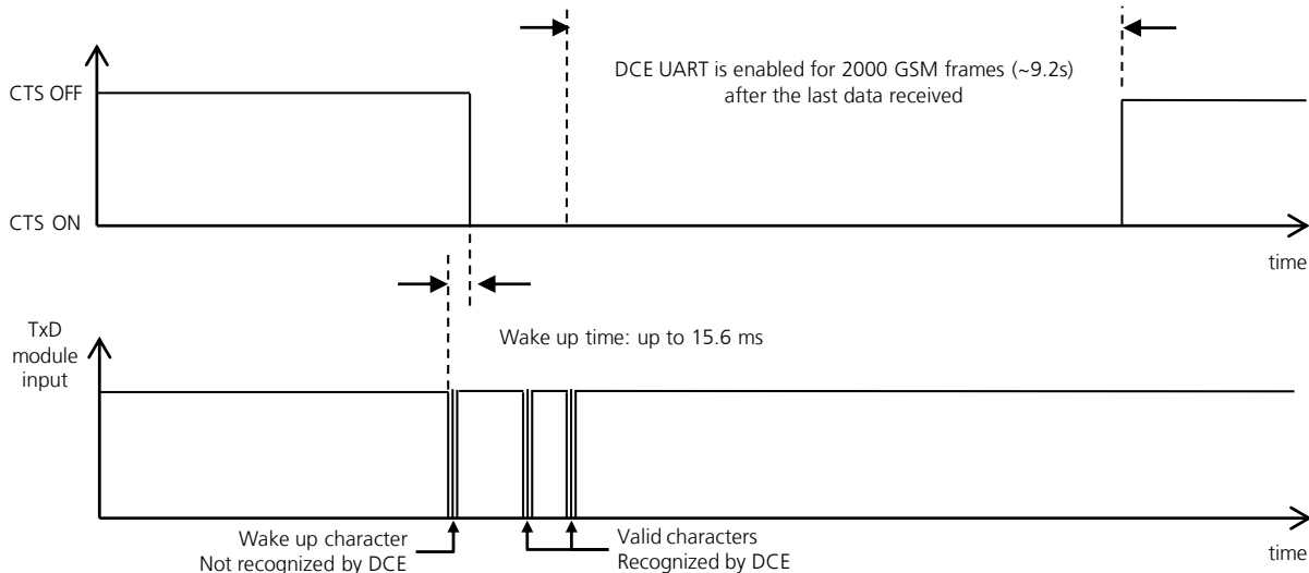
Figure 27: Wake-up via data reception with further communication
