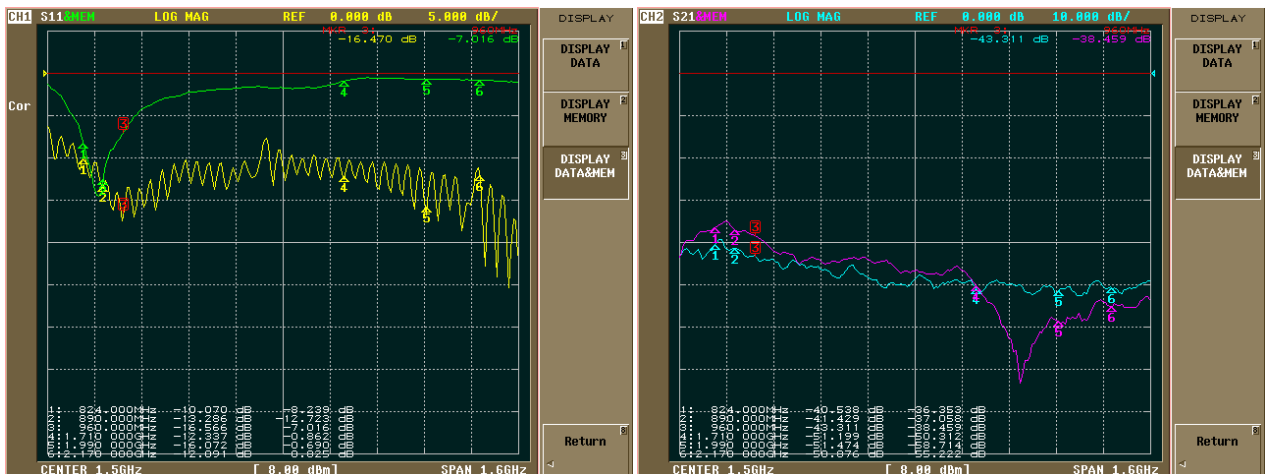
Figure 68: |S_{11}| and |S_{21}| comparison between a 900 MHz tuned half wavelength dipole (green/purple) and a wideband commercial antenna (yellow/cyan)
