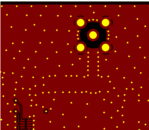
Figure 61: Layer 4 (bottom layer) of u-blox approved interface board for LISA-U modules
