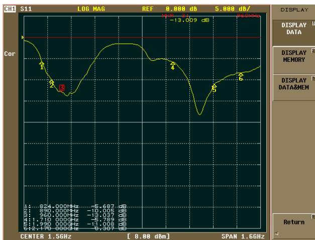
Figure 65: |S_{11}| sample measurement of a penta-band antenna that covers in a small form factor the 4 GSM bands (850 MHz, 900 MHz, 1800 MHz and 1900 MHz) and the UMTS Band I
