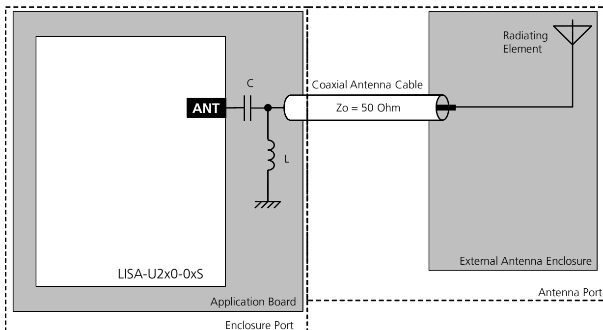
Figure 70: Antenna port ESD immunity protection application circuit for LISA-U2x0-0xS modules
