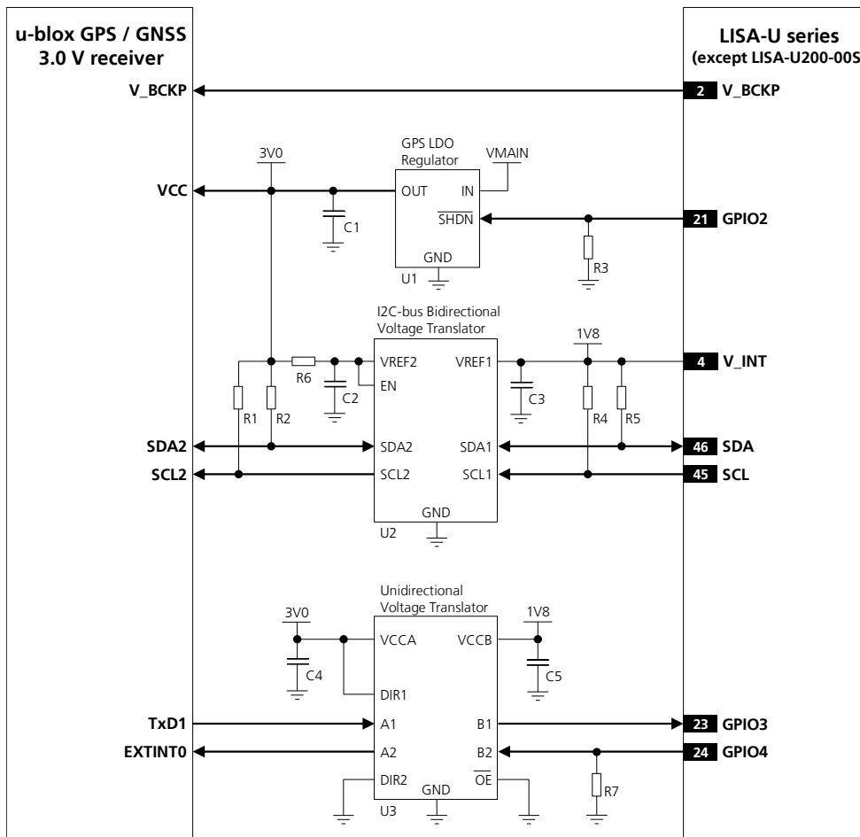
Figure 42: DDC Application circuit for u-blox 3.0 V GPS / GNSS receiver
