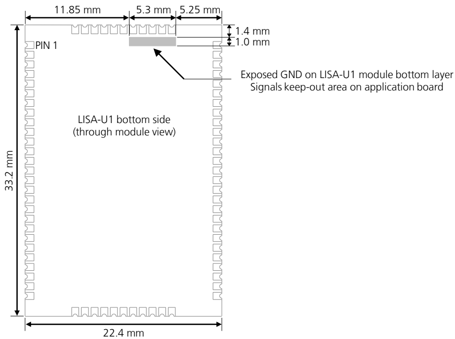
Figure 63: Signals keep-out area on the top layer of the application board, below LISA-U1 series modules
