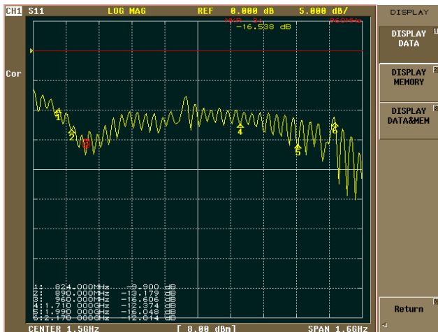
Figure 66: |S_{11}| sample measurement of a wideband antenna
