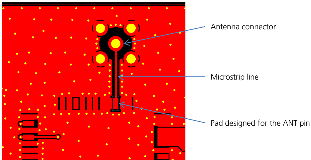
Figure 58: Layer 1 (top layer) of u-blox approved interface board for LISA-U modules
