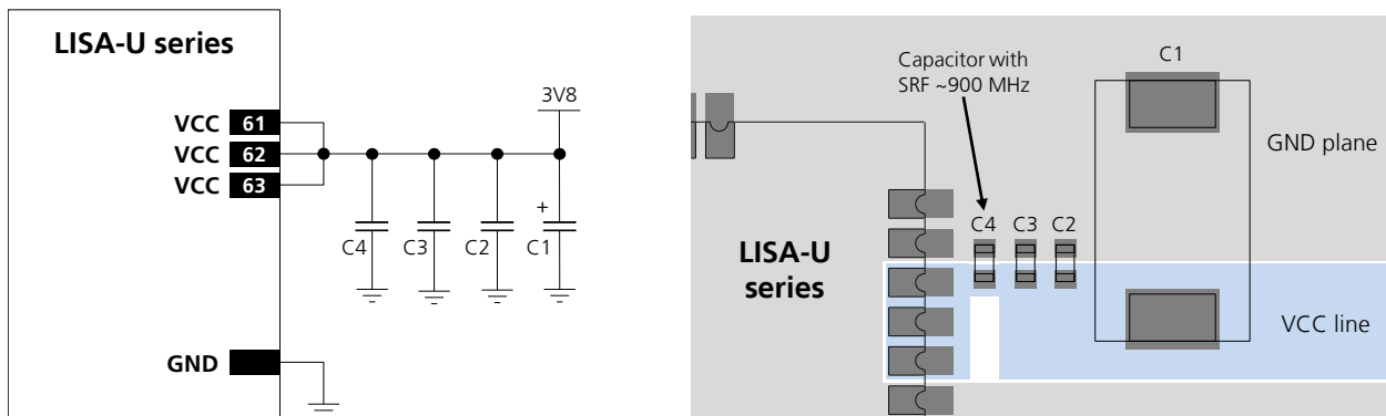
Figure 9: Suggested schematic and layout design for the VCC bypass capacitors to reduce ripple / noise on VCC voltage profile and to avoid undershoot / overshoot on VCC voltage drops
