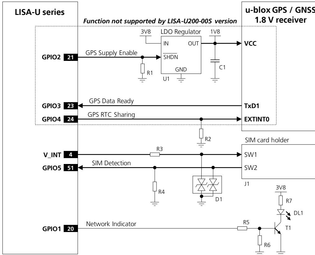
Figure 51: GPIO application circuit
