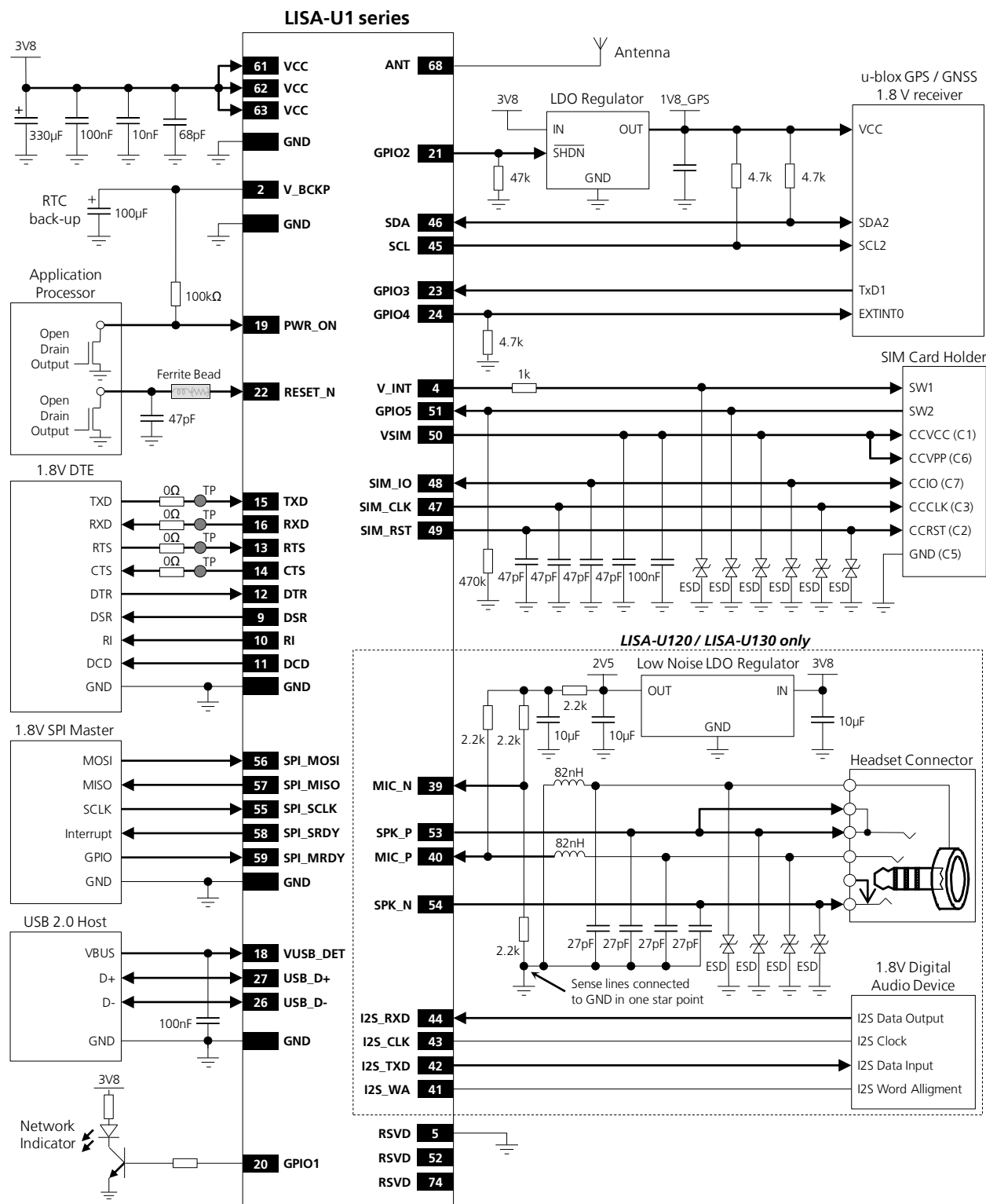
Figure 54: Example of schematic diagram to integrate LISA-U1 series modules in an application board, using all the interfaces
