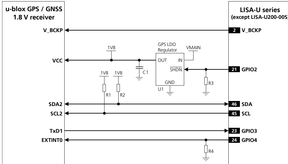
Figure 41: DDC Application circuit for u-blox 1.8 V GPS / GNSS receiver
