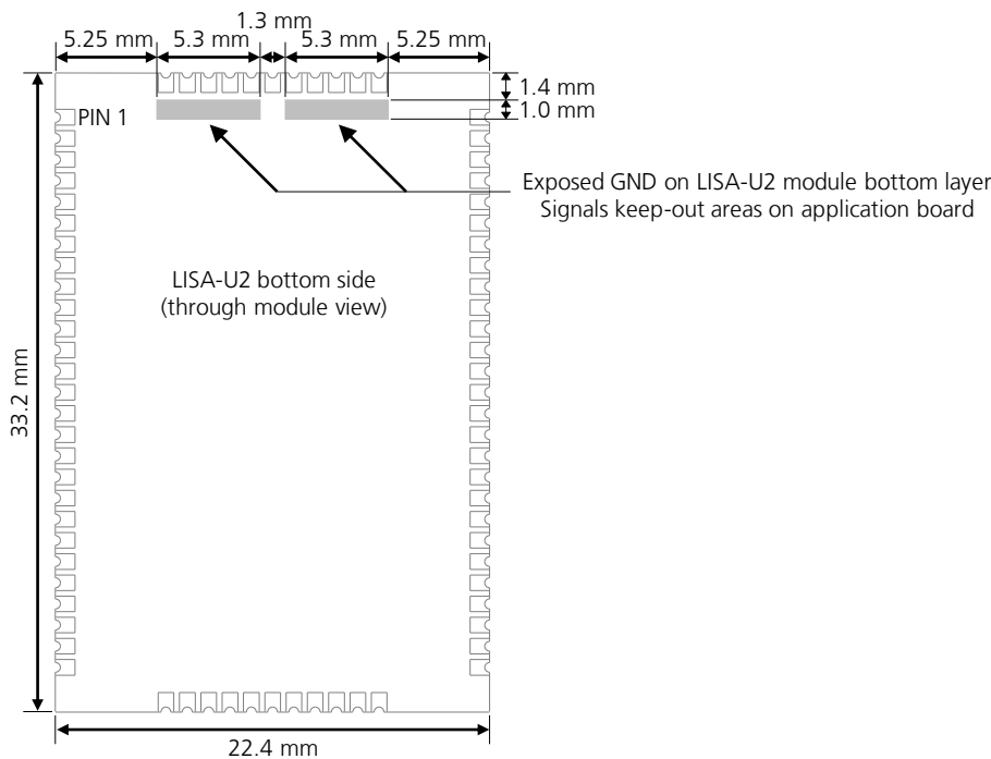
Figure 81: Signals keep-out areas on the top layer of the application board, below LISA-U2 series modules
