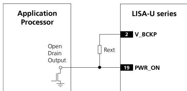
Figure 17: PWR_ON application circuits using an open drain output of an application processor
