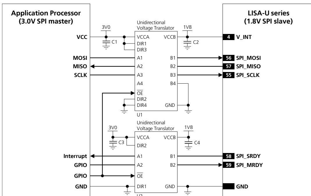
Figure 40: IPC / SPI Interface application circuit connecting LISA-U series 1.8V SPI slave to a 3.0V SPI master
