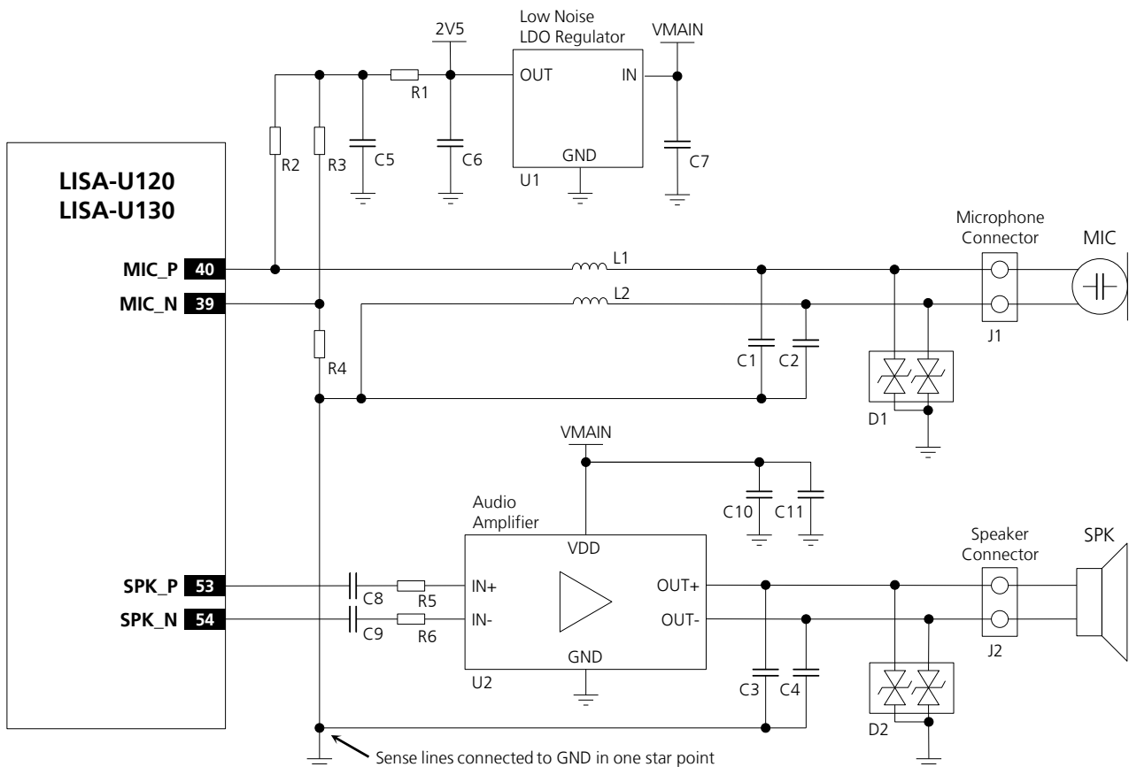
Figure 45: Hands-free mode application circuit
