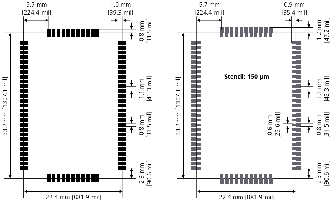
Figure 62: LISA-U modules suggested footprint and paste mask
