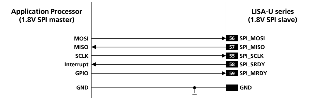
Figure 39: IPC / SPI Interface application circuit connecting LISA-U series 1.8V SPI slave to a 1.8V SPI master
