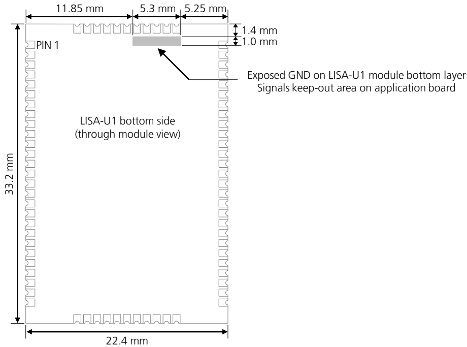
Figure 80: Signals keep-out area on the top layer of the application board, below LISA-U1 series modules
