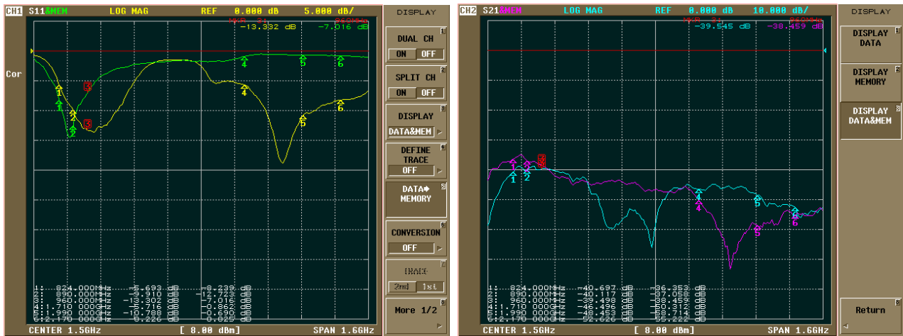
Figure 67: |S_{11}| and |S_{21}| comparison between a 900 MHz tuned half wavelength dipole (green/purple) and a penta-band internal antenna (yellow/cyan)
