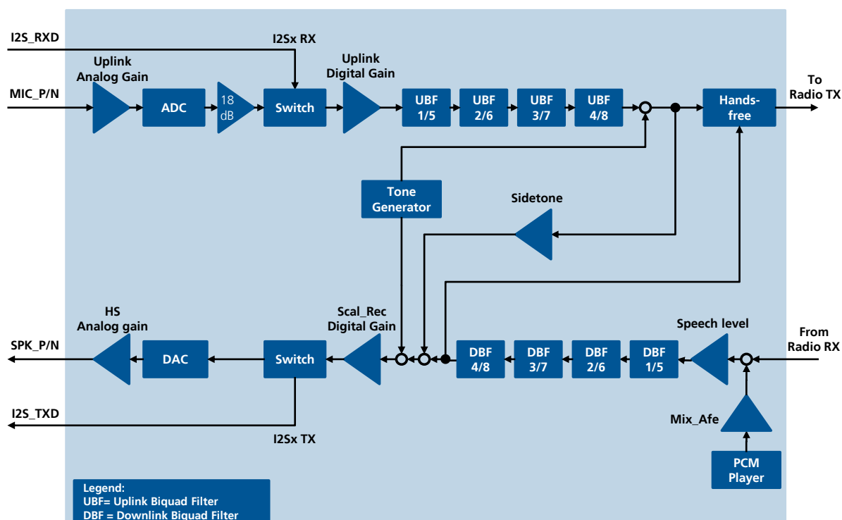
Figure 49: Audio processing system of LISA-U120 and LISA-U130
