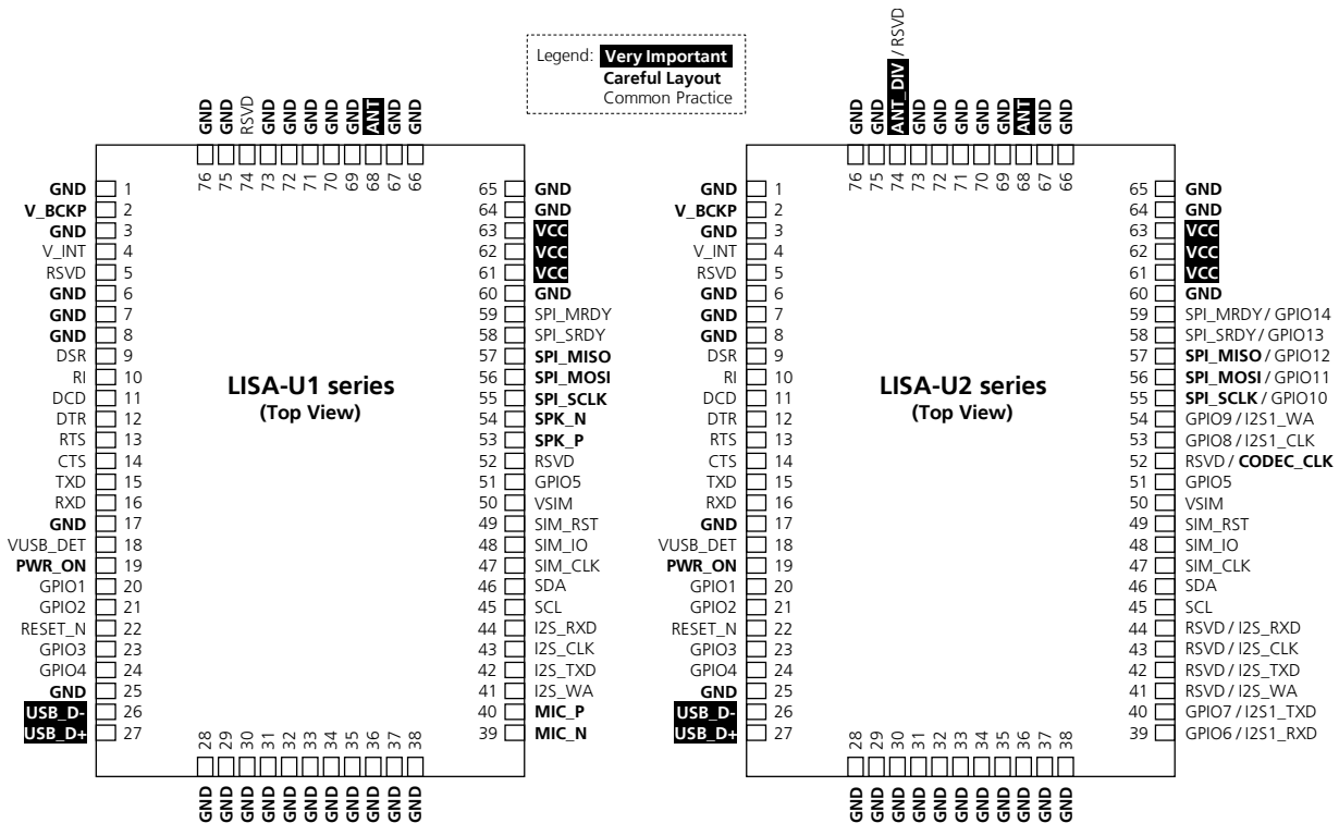
Figure 56: LISA-U1 and LISA-U2 series modules pin-out (top view) with ranked importance for layout design
