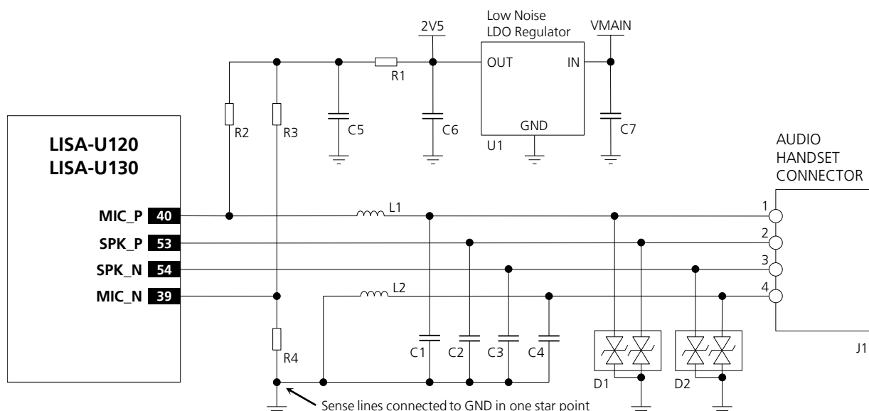
Figure 44: Handset mode application circuit
