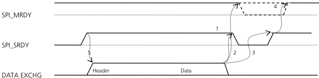
Figure 38: Data transfer terminated and then restarted by LISA-U module (slave)
