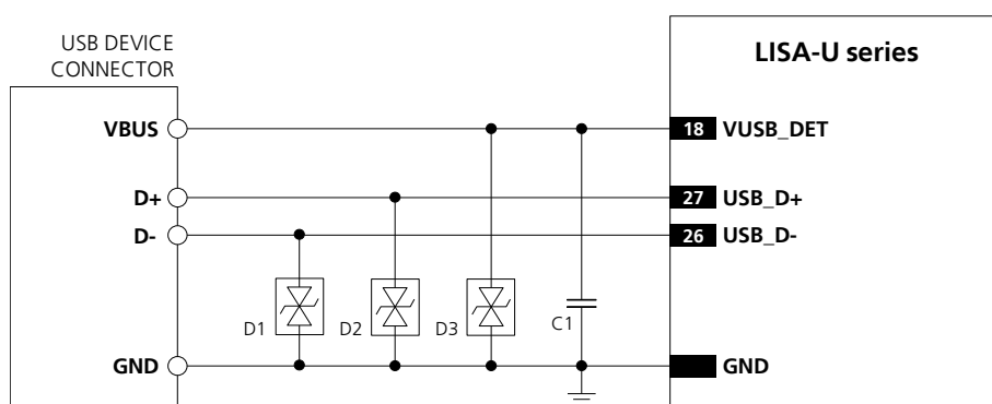
Figure 34: USB Interface application circuit
