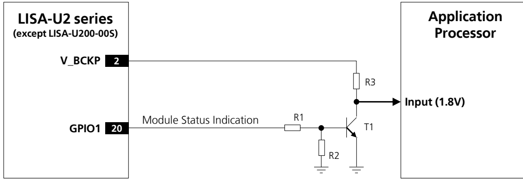
Figure 52: Module status indication application circuit
