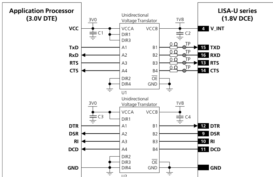
Figure 29: UART interface application circuit with complete V.24 link in DTE/DCE serial communication (3.0 V DTE)
