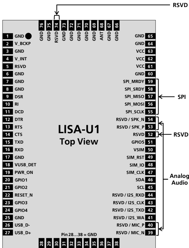
Figure 78: LISA-U1 series pin assignment
