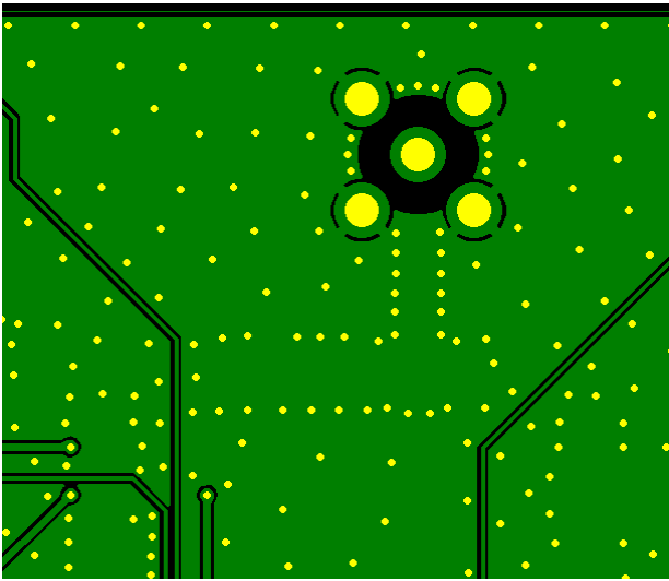
Figure 60: Layer 3 (inner layer) of u-blox approved interface board for LISA-U modules
