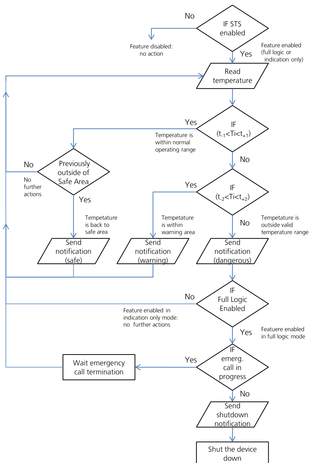
Figure 72: Smart Temperature Supervisor (STS) flow diagram
