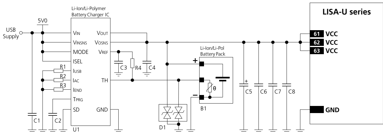
Figure 10: Li-Ion (or Li-Polymer) battery charging application circuit
