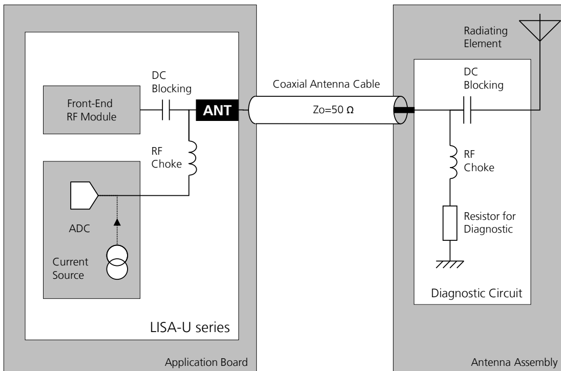
Figure 69: Antenna detection circuit and antenna with diagnostic resistor
