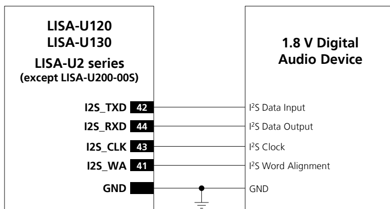
Figure 47: I 2 S interface application circuit with a generic digital audio device
