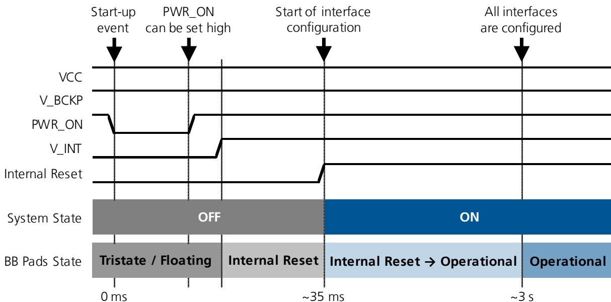
Figure 18: LISA-U series power-on sequence description
