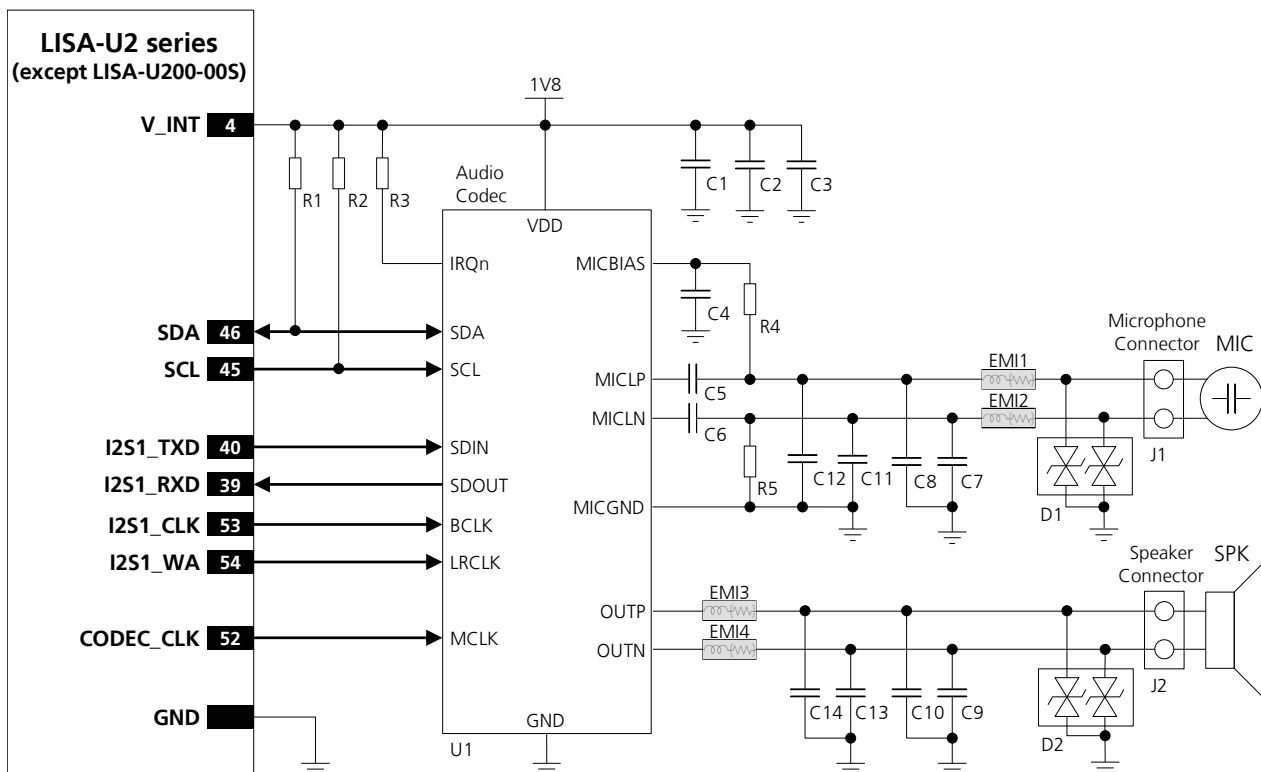
Figure 48: I 2 S interface application circuit with an external audio codec to provide voice capability
