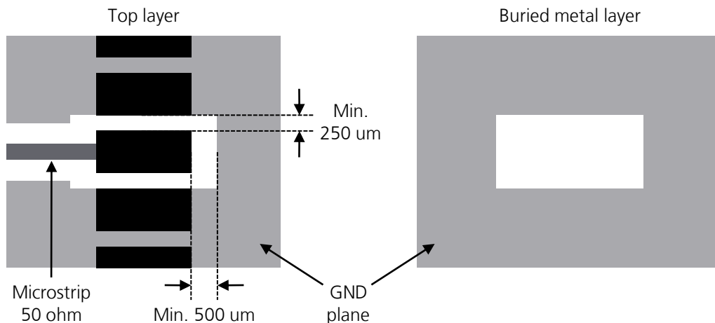
Figure 57: GND keep-out area on top layer around ANT and ANT_DIV pads and on buried layer below ANT and ANT_DIV pads
